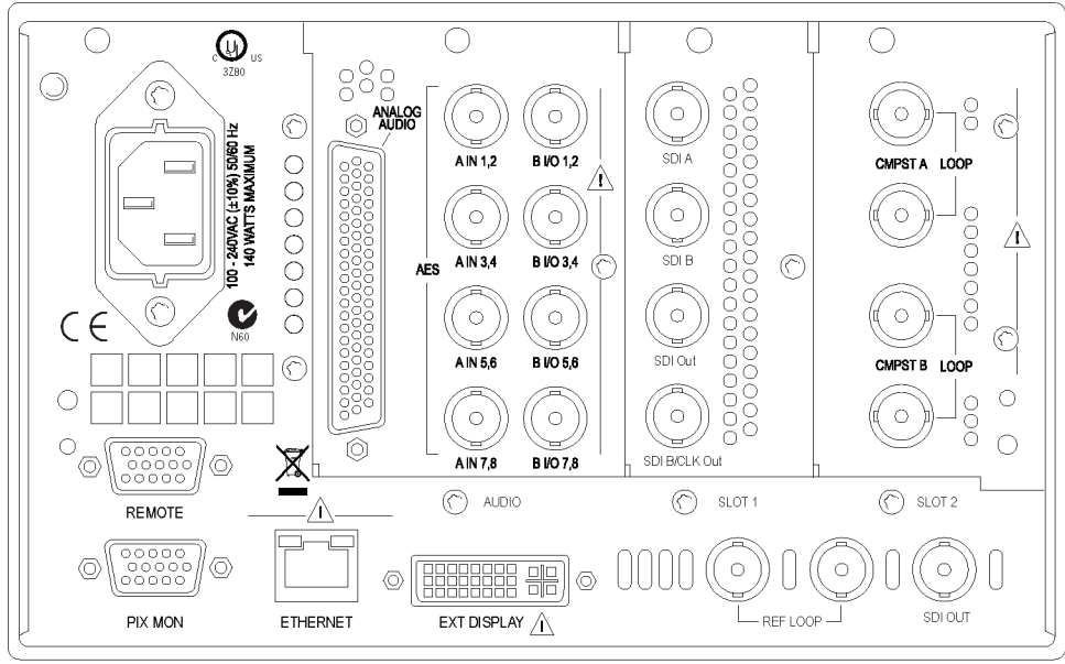
Rear-panel
